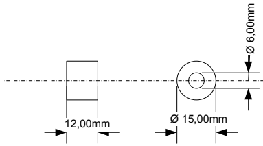
Distanzhülse
